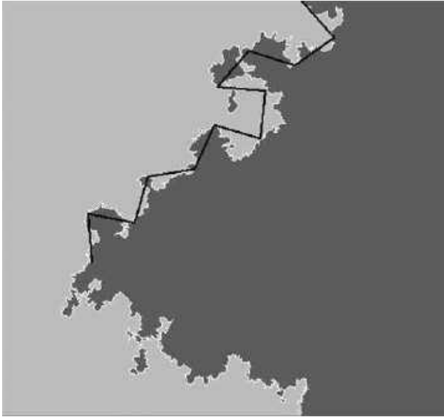
FIG. 6.9. Synthetic fractal coastline (courtesy of P. Trunfio).
